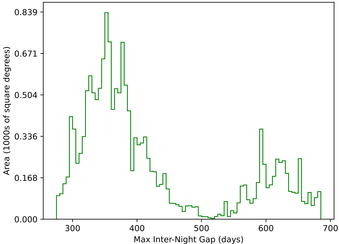
too_elab_r256_d2_ugrizy_v3.4_10yrs WFD g band: Max Inter-Night Gap
