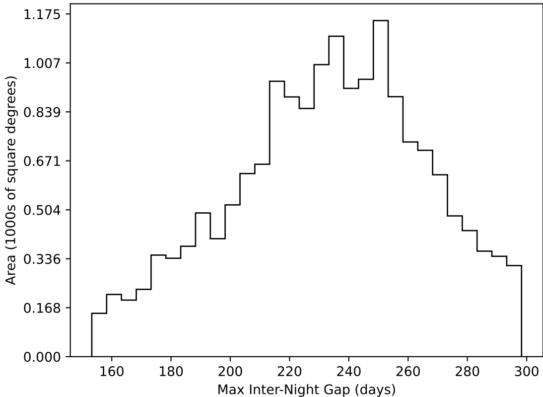
too_elab_r256_d2_ugrizy_v3.4_10yrs WFD all bands: Max Inter-Night Gap
