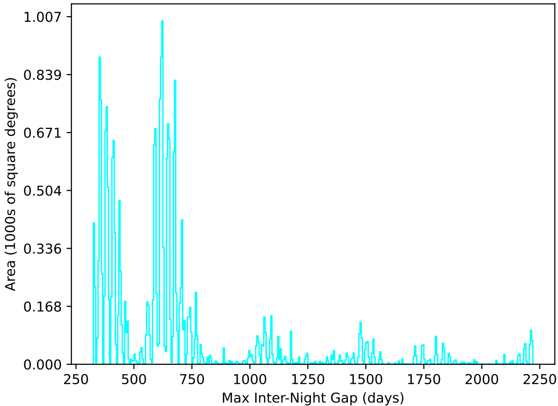
too_elab_r256_d2_ugrizy_v3.4_10yrs All sky u band: Max Inter-Night Gap
