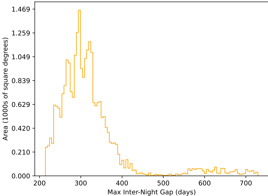
too_elab_r256_d2_ugrizy_v3.4_10yrs All sky r band: Max Inter-Night Gap
