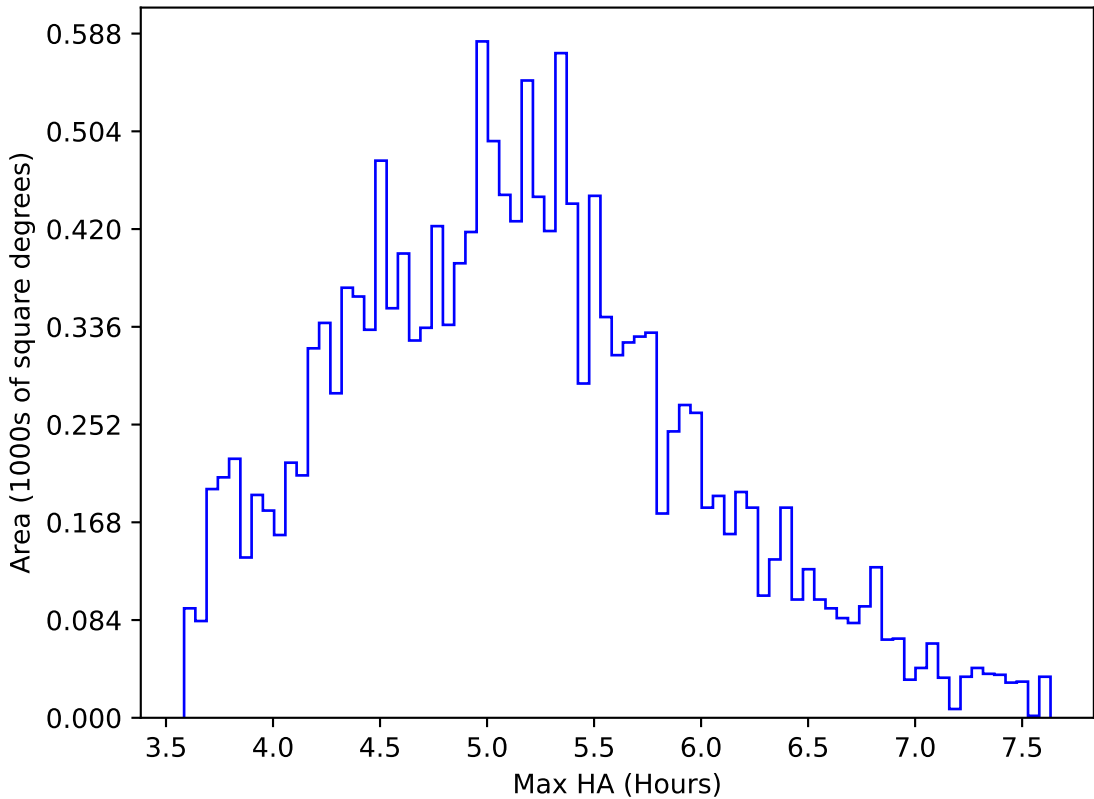
too_elab_r256_d2_ugrizy_v3.4_10yrs WFD all bands: Max HA
