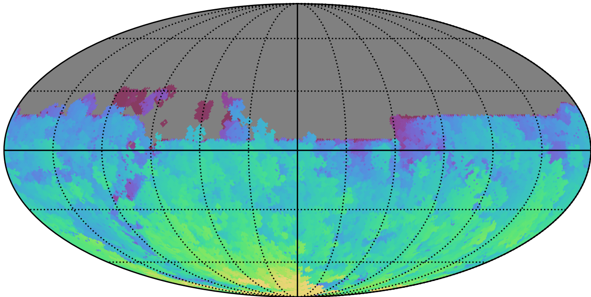
too_elab_r256_d2_ugrizy_v3.4_10yrs All sky u band: Max HA
