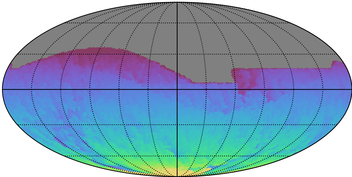
too_elab_r256_d2_ugrizy_v3.4_10yrs All sky all bands: Max HA
