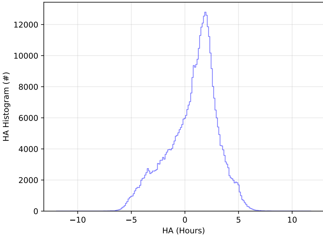
too_elab_r256_d2_ugrizy_v3.4_10yrs WFD z band: HA Histogram
