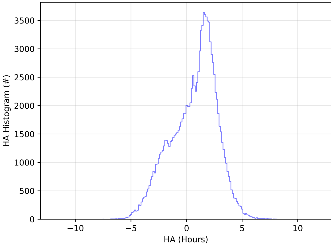
too_elab_r256_d2_ugrizy_v3.4_10yrs WFD u band: HA Histogram
