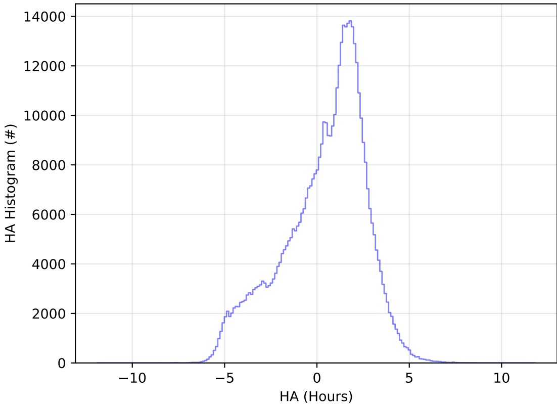
too_elab_r256_d2_ugrizy_v3.4_10yrs WFD r band: HA Histogram
