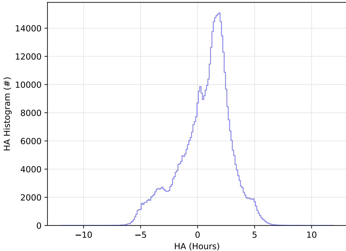
too_elab_r256_d2_ugrizy_v3.4_10yrs WFD i band: HA Histogram
