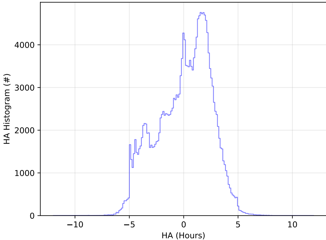
too_elab_r256_d2_ugrizy_v3.4_10yrs WFD g band: HA Histogram
