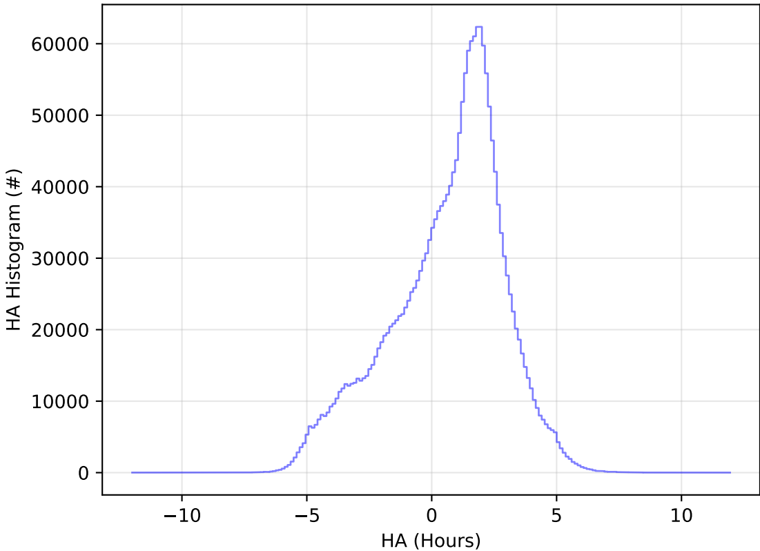
too_elab_r256_d2_ugrizy_v3.4_10yrs WFD all bands: HA Histogram
