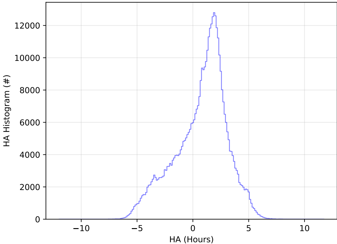
too_elab_r256_d2_ugrizy_v3.4_10yrs All sky z band: HA Histogram
