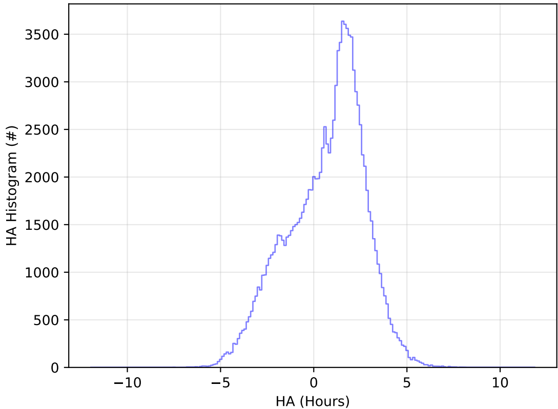
too_elab_r256_d2_ugrizy_v3.4_10yrs All sky u band: HA Histogram
