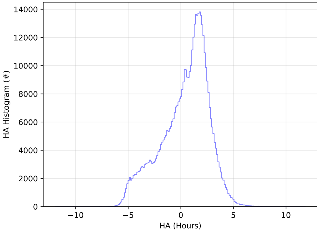
too_elab_r256_d2_ugrizy_v3.4_10yrs All sky r band: HA Histogram
