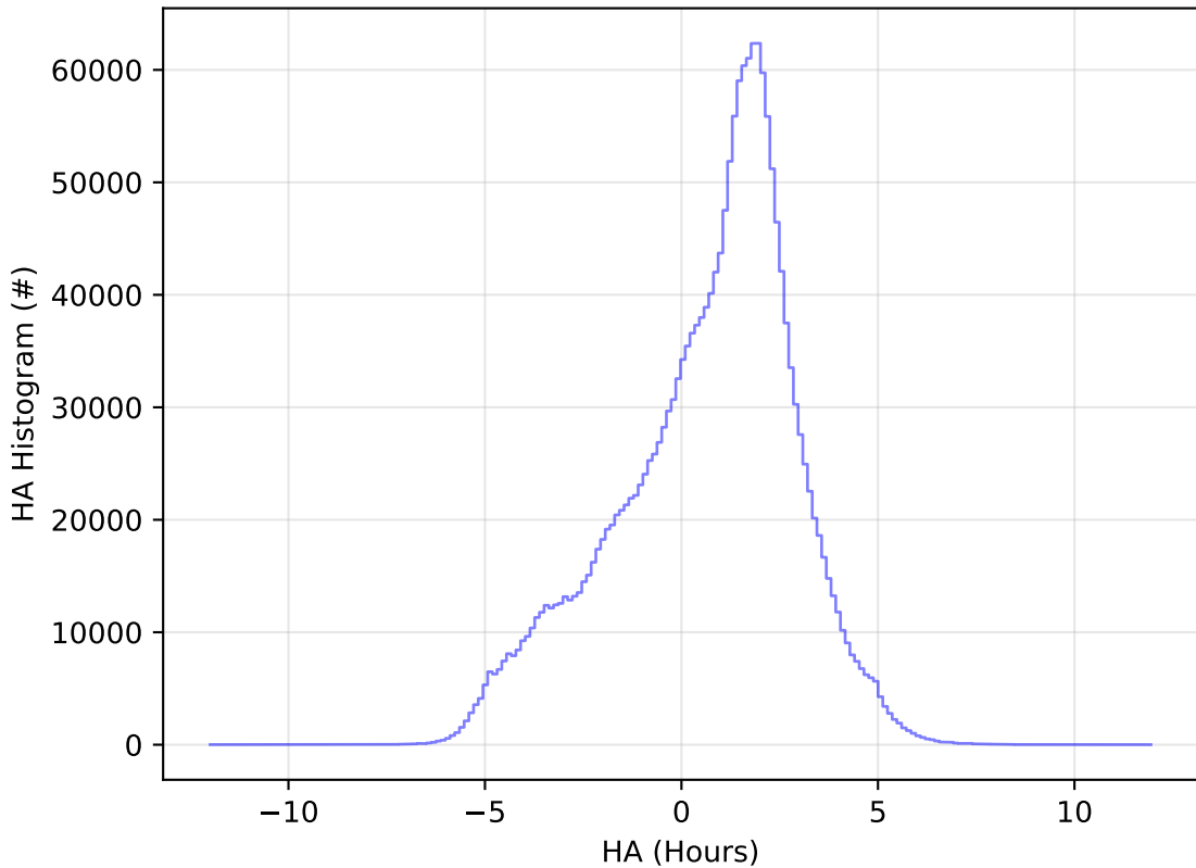
too_elab_r256_d2_ugrizy_v3.4_10yrs All sky all bands: HA Histogram
