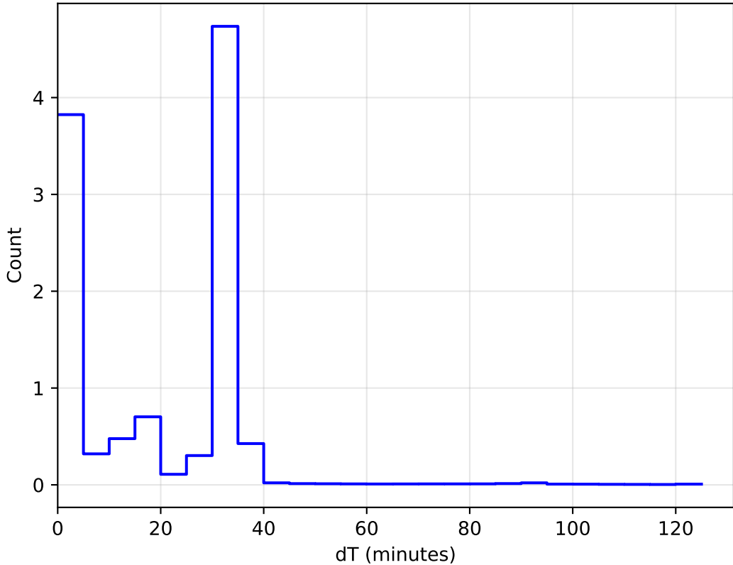
too_elab_r256_d2_ugrizy_v3.4_10yrs WFD: DeltaT Histogram 1e6
