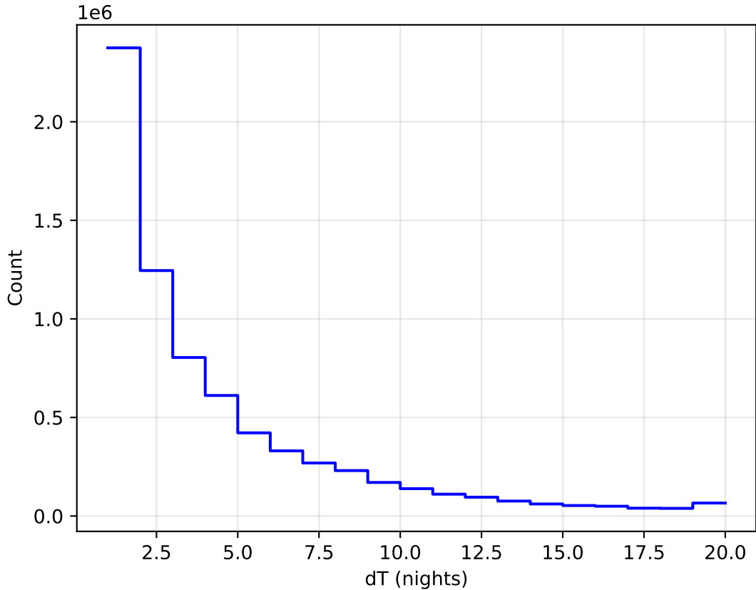
too_elab_r256_d2_ugrizy_v3.4_10yrs WFD all bands: DeltaNight Histogram
