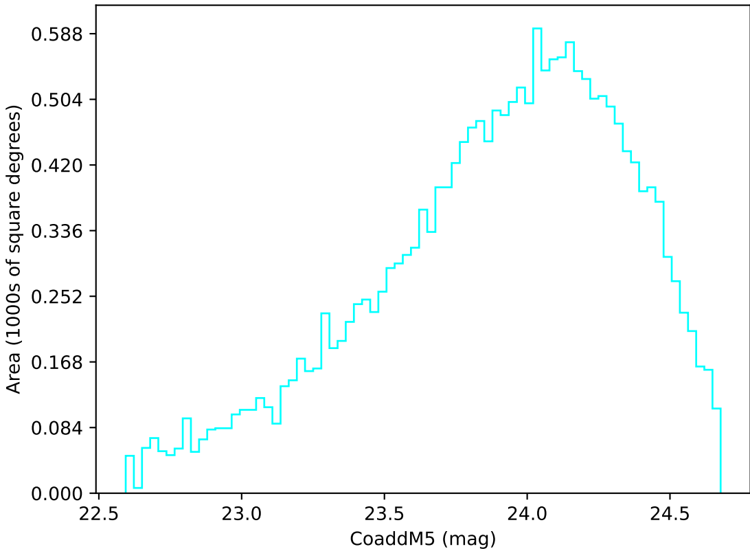
too_elab_r256_d2_ugrizy_v3.4_10yrs Yr 3-4 u band: CoaddM5
