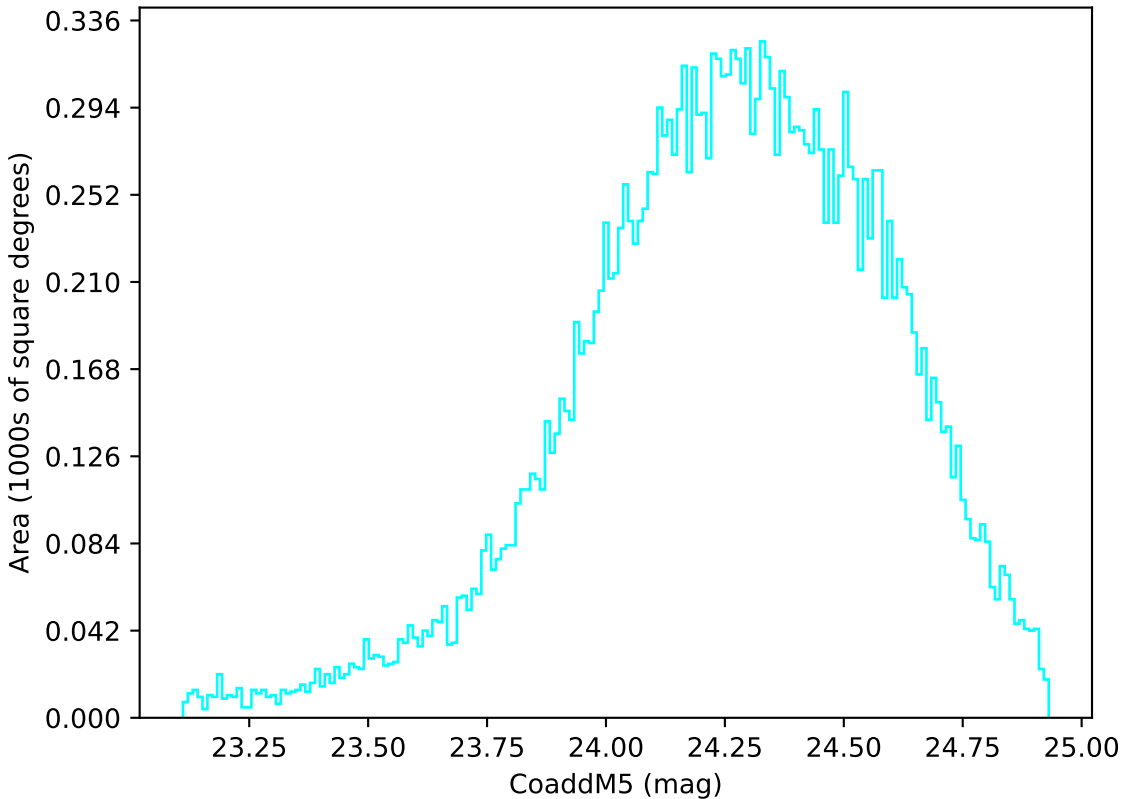
too_elab_r256_d2_ugrizy_v3.4_10yrs Yr 1 u band: CoaddM5
