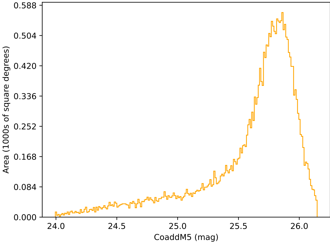
too_elab_r256_d2_ugrizy_v3.4_10yrs Yr 1 r band: CoaddM5
