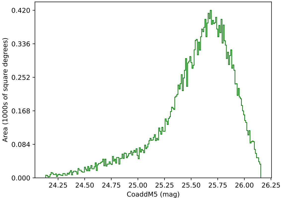
too_elab_r256_d2_ugrizy_v3.4_10yrs Yr 1 g band: CoaddM5
