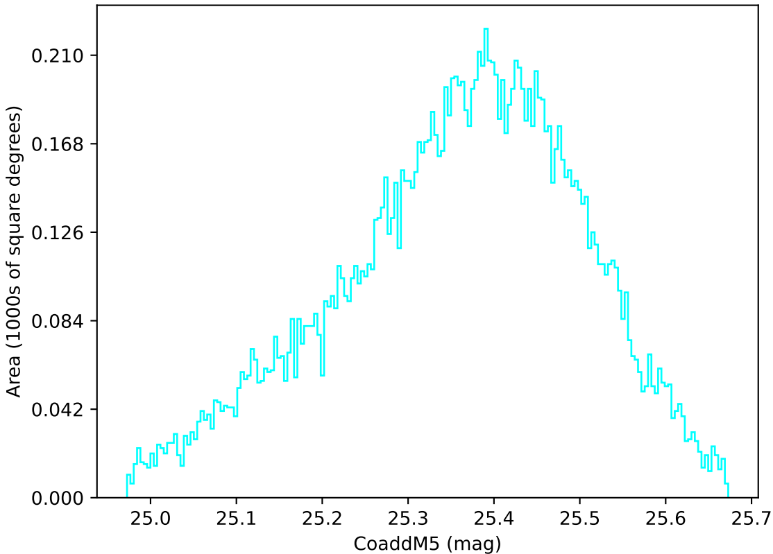
too_elab_r256_d2_ugrizy_v3.4_10yrs WFD u band: CoaddM5
