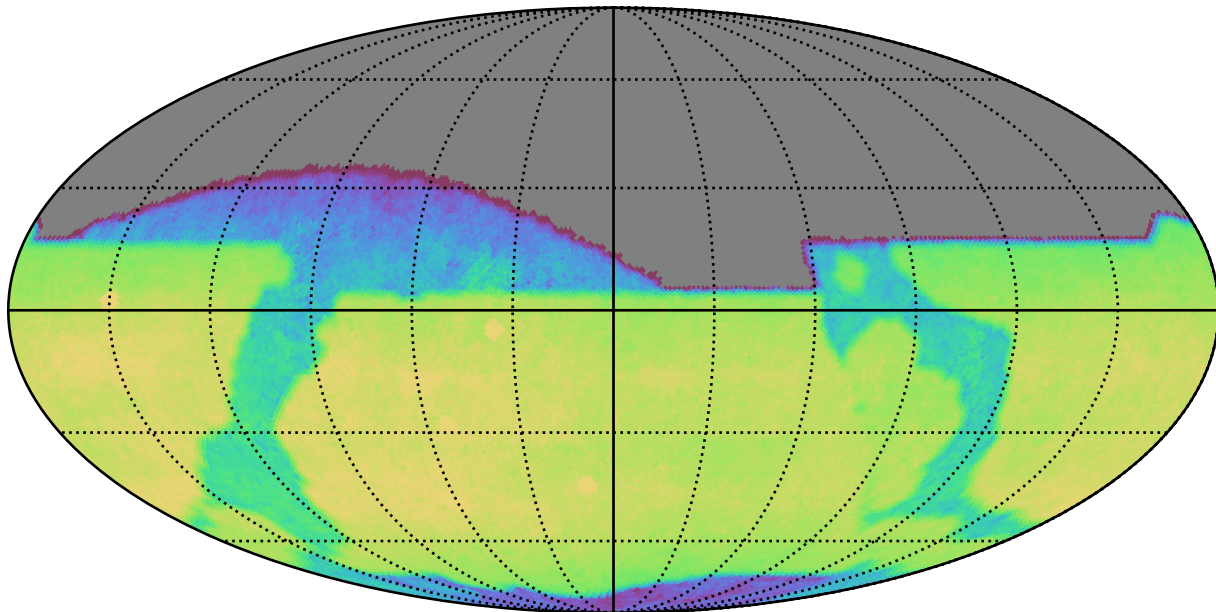
too_elab_r256_d2_ugrizy_v3.4_10yrs All sky z band: CoaddM5
