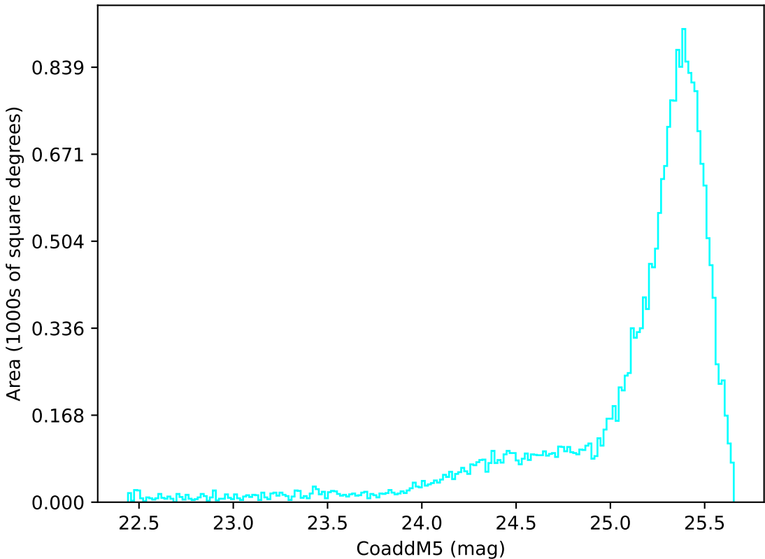
too_elab_r256_d2_ugrizy_v3.4_10yrs All sky u band: CoaddM5
