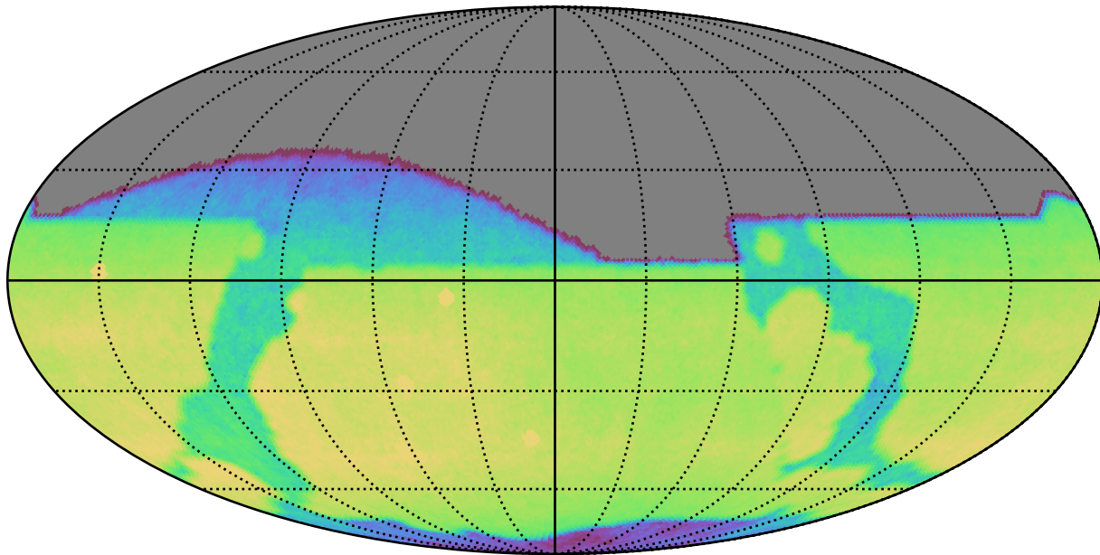
too_elab_r256_d2_ugrizy_v3.4_10yrs All sky r band: CoaddM5
