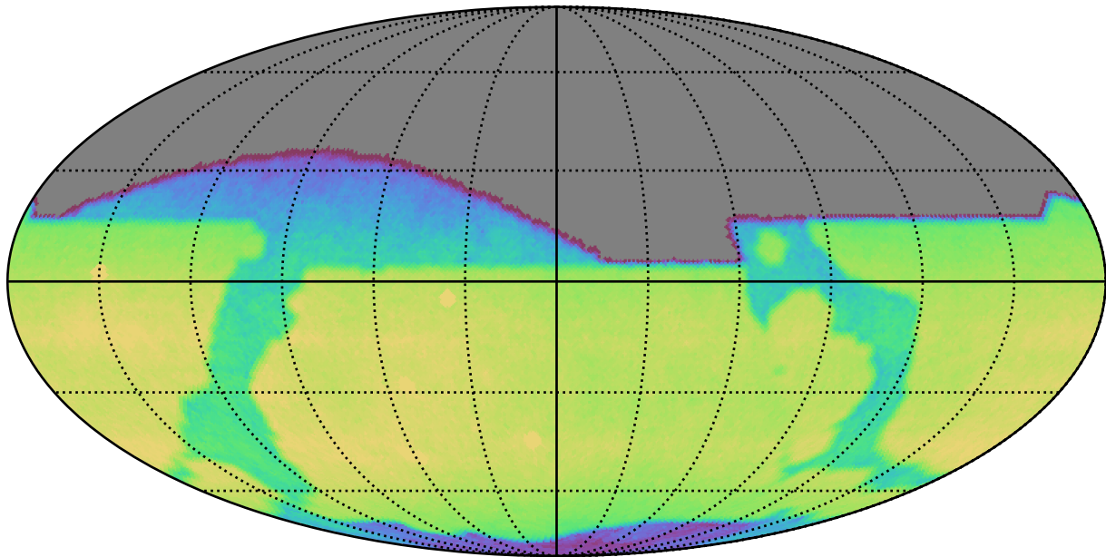
too_elab_r256_d2_ugrizy_v3.4_10yrs All sky i band: CoaddM5
