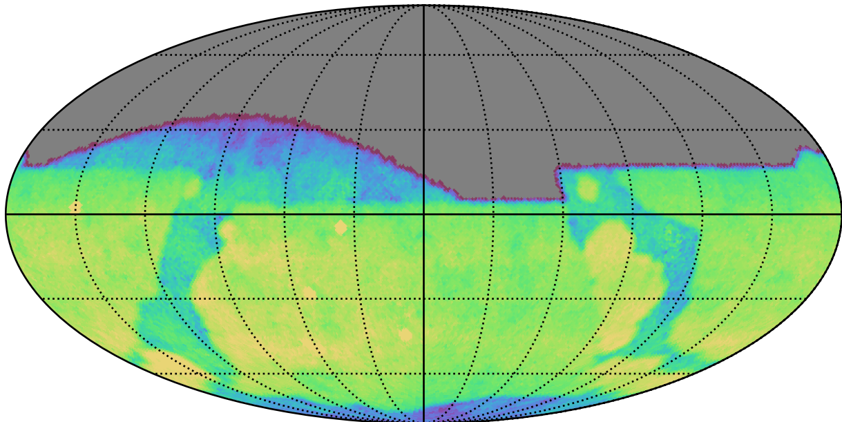
too_elab_r256_d2_ugrizy_v3.4_10yrs All sky g band: CoaddM5
