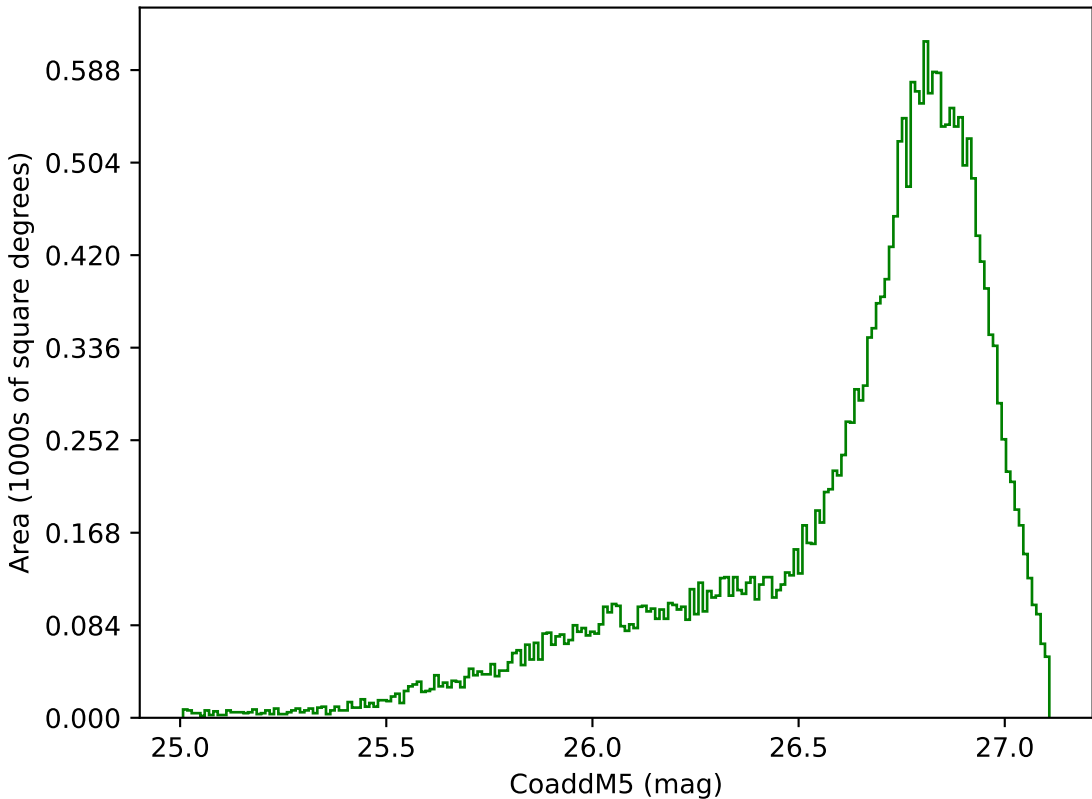
too_elab_r256_d2_ugrizy_v3.4_10yrs All sky g band: CoaddM5
