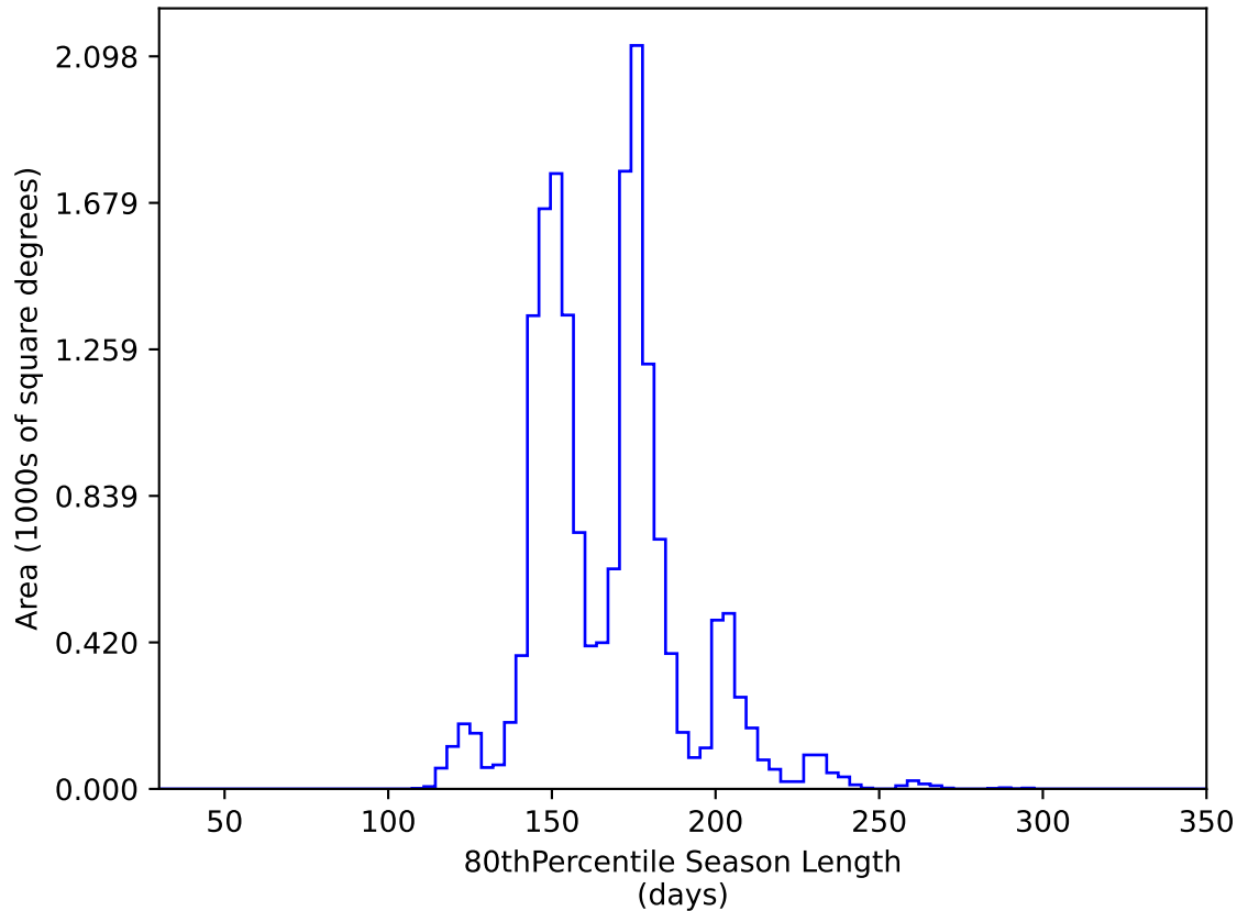
too_elab_r256_d2_ugrizy_v3.4_10yrs WFD y band: 80thPercentile Season Length
