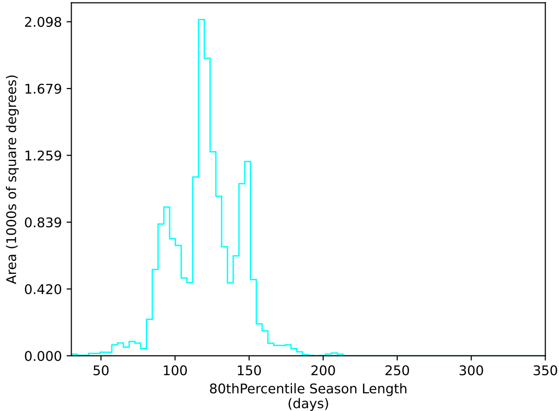
too_elab_r256_d2_ugrizy_v3.4_10yrs WFD u band: 80thPercentile Season Length
