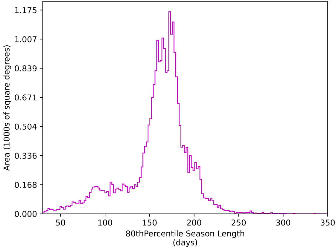
too_elab_r256_d2_ugrizy_v3.4_10yrs All sky z band: 80thPercentile Season Length
