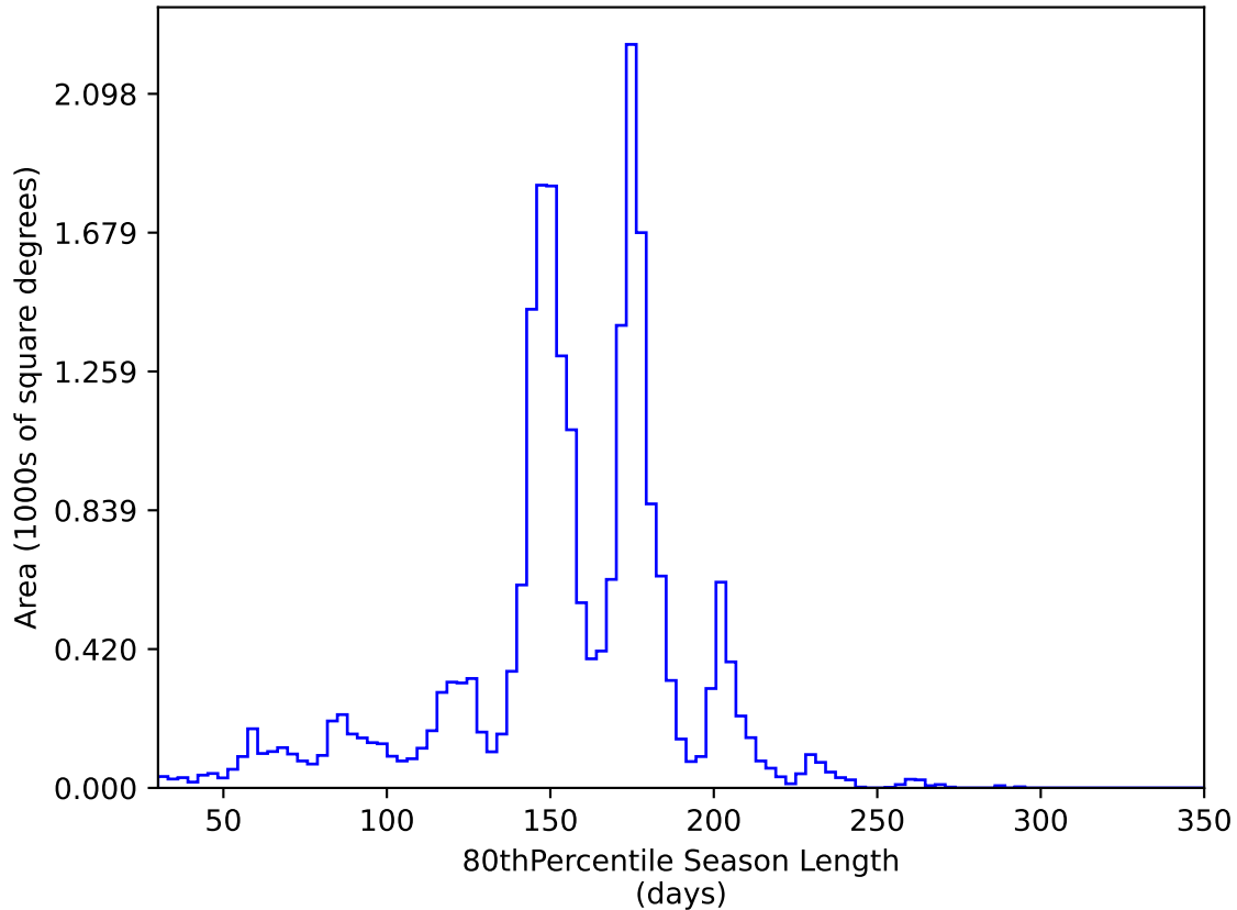
too_elab_r256_d2_ugrizy_v3.4_10yrs All sky y band: 80thPercentile Season Length
