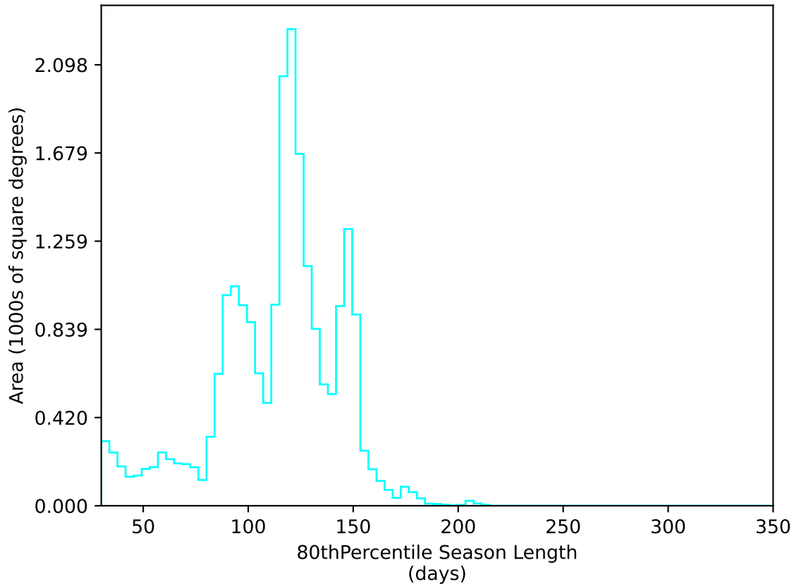
too_elab_r256_d2_ugrizy_v3.4_10yrs All sky u band: 80thPercentile Season Length
