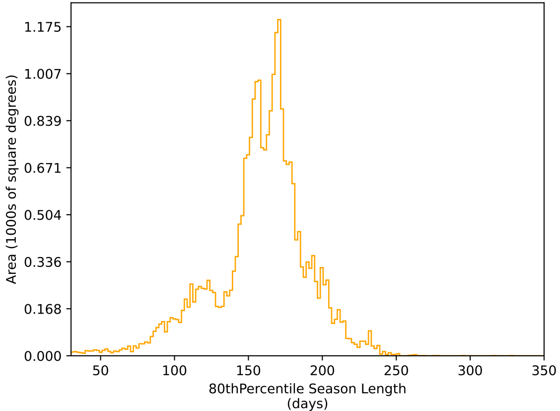
too_elab_r256_d2_ugrizy_v3.4_10yrs All sky r band: 80thPercentile Season Length
