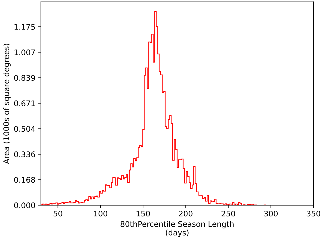
too_elab_r256_d2_ugrizy_v3.4_10yrs All sky i band: 80thPercentile Season Length
