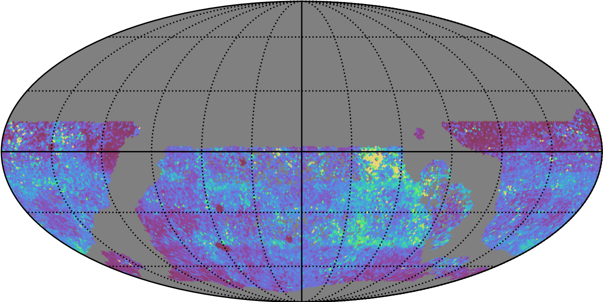
too_elab_r256_d2_ugrizy_v3.4_10yrs WFD y band: 75th Percentile Intranight Timespan
