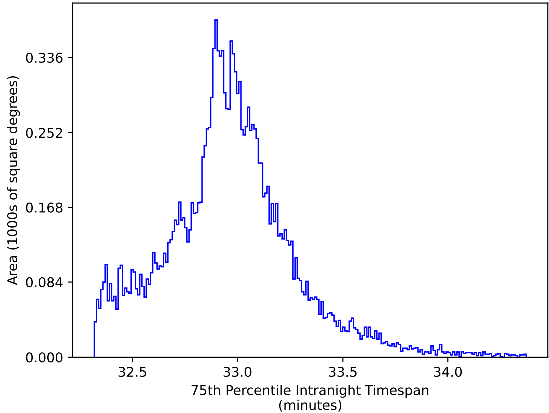
too_elab_r256_d2_ugrizy_v3.4_10yrs WFD y band: 75th Percentile Intranight Timespan
