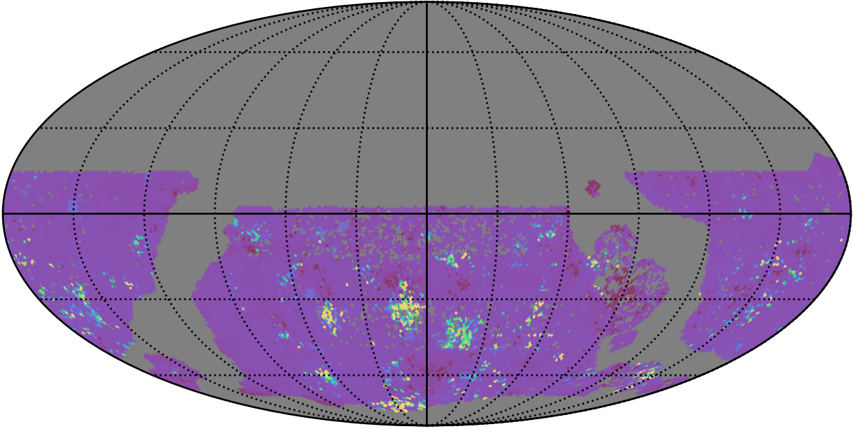
too_elab_r256_d2_ugrizy_v3.4_10yrs WFD ug bands: 75th Percentile Intranight Timespan
