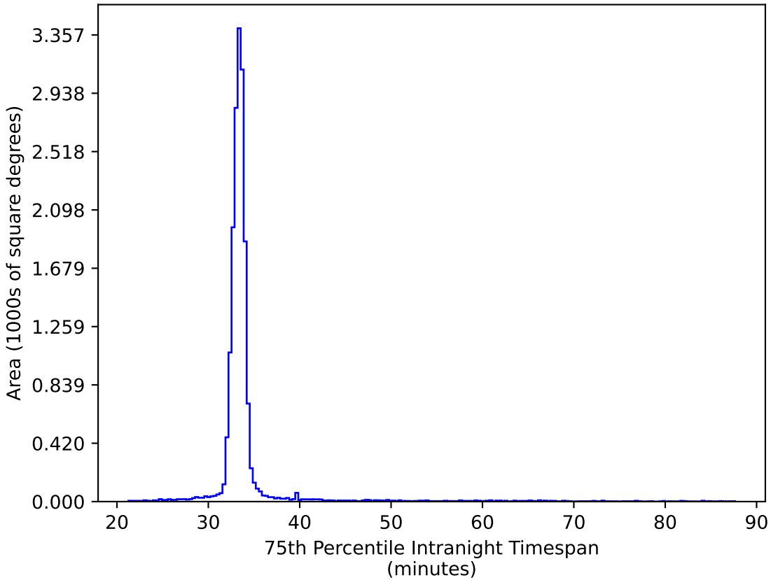
too_elab_r256_d2_ugrizy_v3.4_10yrs WFD ug bands: 75th Percentile Intranight Timespan
