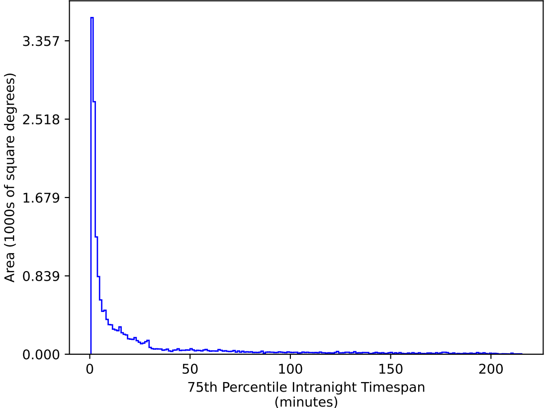
too_elab_r256_d2_ugrizy_v3.4_10yrs WFD u band: 75th Percentile Intranight Timespan
