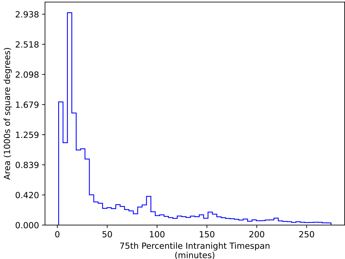
too_elab_r256_d2_ugrizy_v3.4_10yrs WFD r band: 75th Percentile Intranight Timespan
