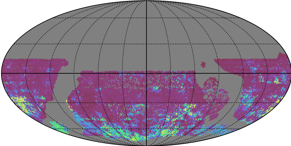
too_elab_r256_d2_ugrizy_v3.4_10yrs WFD i band: 75th Percentile Intranight Timespan
