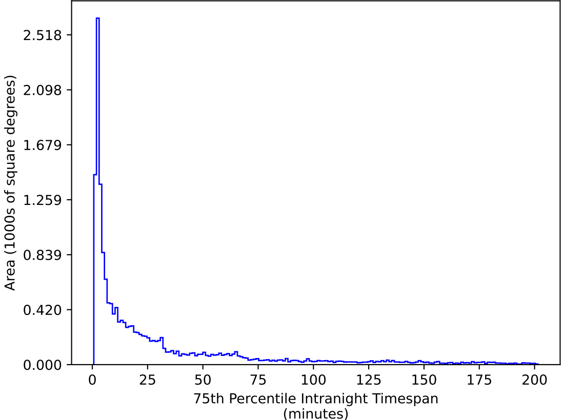
too_elab_r256_d2_ugrizy_v3.4_10yrs WFD g band: 75th Percentile Intranight Timespan
