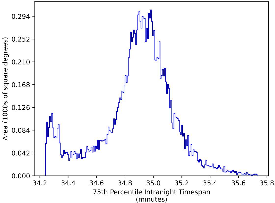
too_elab_r256_d2_ugrizy_v3.4_10yrs WFD all bands: 75th Percentile Intranight Timespan
