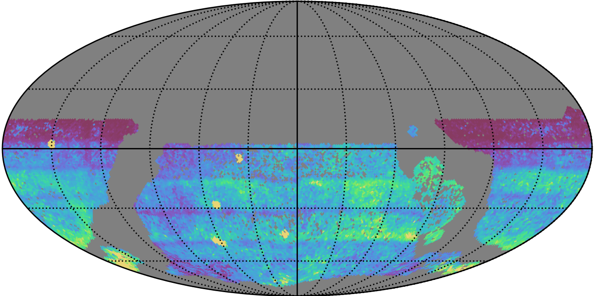
too_elab_r256_d2_ugrizy_v3.4_10yrs WFD: 75th Percentile Intranight Timespan
