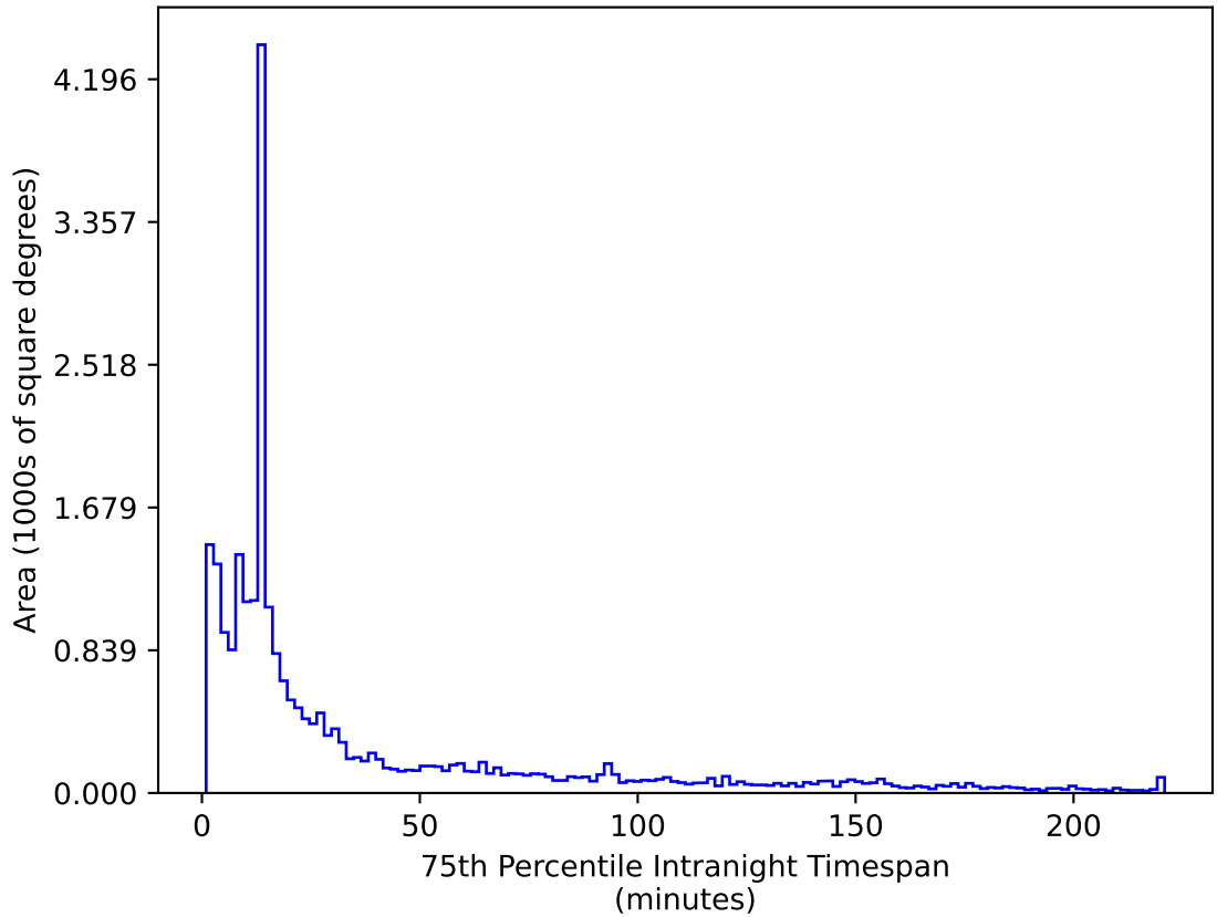
too_elab_r256_d2_ugrizy_v3.4_10yrs All sky z band: 75th Percentile Intranight Timespan
