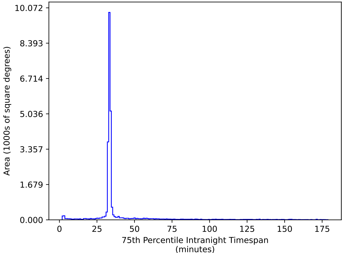
too_elab_r256_d2_ugrizy_v3.4_10yrs All sky ug bands: 75th Percentile Intranight Timespan
