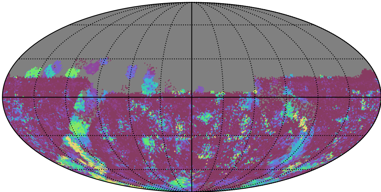
too_elab_r256_d2_ugrizy_v3.4_10yrs All sky u band: 75th Percentile Intranight Timespan
